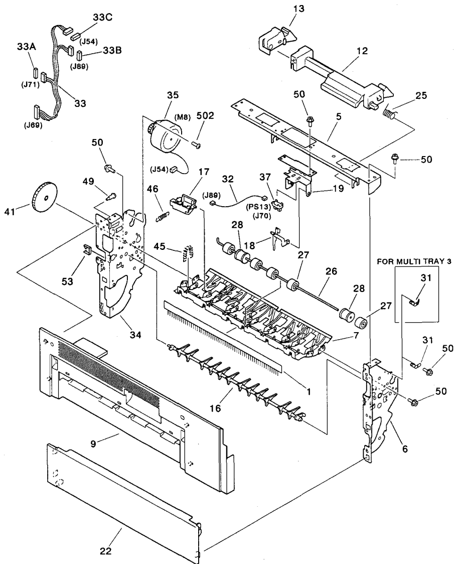
FIGURE Q35 DELIVERY ASSEMBLY (GP215) (1/2) 排紙部 (GP215) (1/2)
